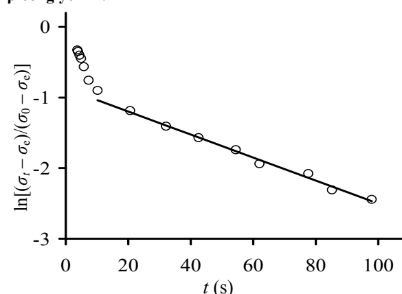
Fig. 2 Plot of \ln[(\sigma_t - \sigma_c)/(\sigma_0 - \sigma_c)] versus t the experimental data of \beta -conglycinin ( \circ ) and as proposed by Kitabatake and Doi [9], corresponding to \beta -conglycinin.
