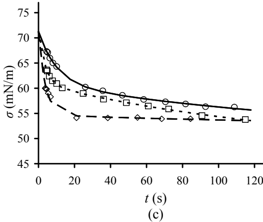
Fig. 5 (a) Curves of surface tension versus time of the experimental data for \alpha -lactalbumin ( \circ ) and \beta -lactoglobulin ( \square ), and the respective curves considered according to Eq. (16) for the same data; (b) curves of surface tension versus time of the experimental data for \beta -conglycinin ( \circ ), glycinin ( \square ) and hemoglobin ( \diamond ), and the respective estimated curves based on Eq. (16); (c) curves of surface tension versus time for the experimental data of lysozyme ( \circ ), bovine serum albumin ( \square ) and \beta -casein ( \diamond ), and the respective estimated curves based on Eq. (16) for the same data.
