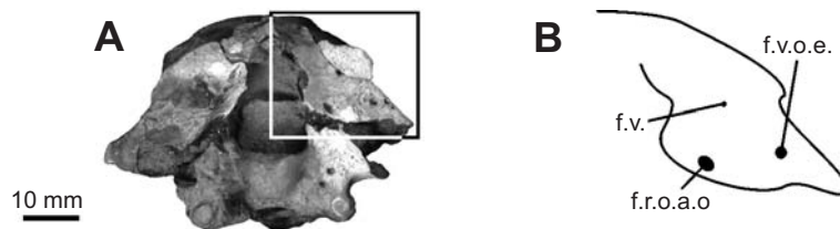
Fig. 7. Details of the cranial foramina in occipital view: A. MLP 12-I-20-1. B. Schematic detail of the sector pointed by the square: f.r.o.a.o. – foramen rami occipitalis arteriae ophtalmica , f.v. – foramen vein , f.v.o.e. – foramen vena occipitalis externa .
