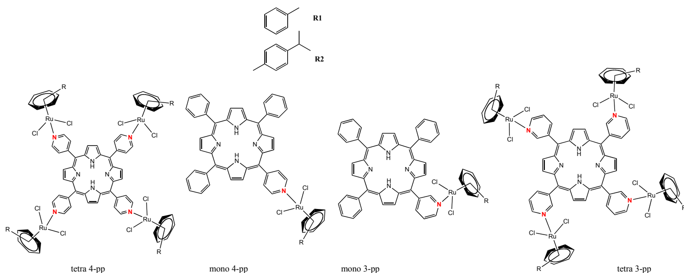
Fig. (19). Arene ligand derivation in monopyritylporphyrin (mpp) and tetrapyritylporphyrin (tpp) compounds.
