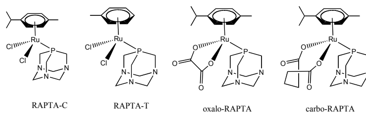
Fig. (15). Chemical structure of RAPTA derivatives.
