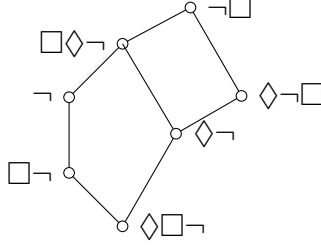
Figure 16: The negative modalities in the S-extension
