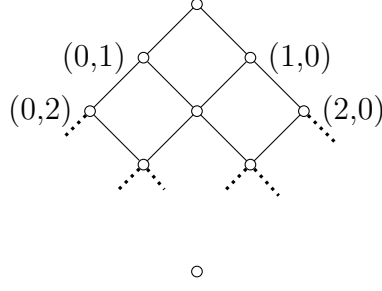
Figure 12: A Gödel algebra where \Diamond does not exist
