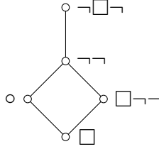
Figure 17: The positive modalities in the distributive S-extension
