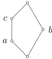
Figure 3: The pentagon
