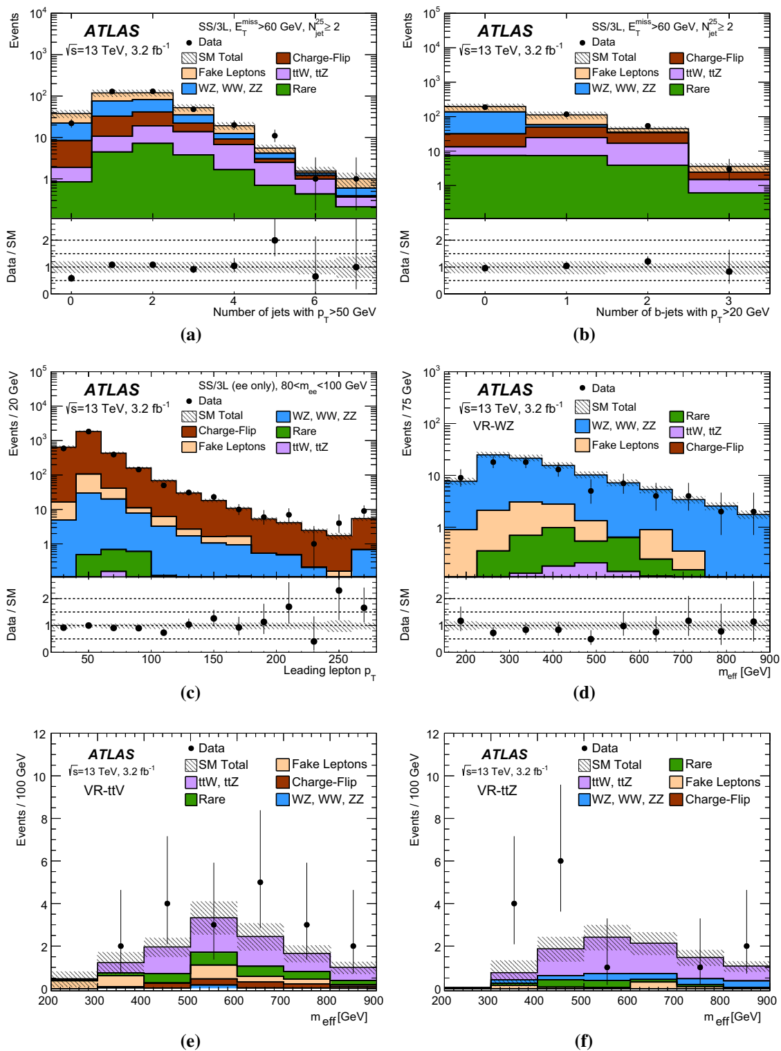
Fig. 2 Distributions of kinematic variables after a SS/3L selection including a , b E_T^{miss} > 60 GeV and N_{jet}^{25} \geq 2 , c a b -jet veto and 80 < m_{\ell\ell} < 100 GeV, and d-f distributions in the validation regions. The statistical uncertainties in the background prediction are included in the uncertainty band, as well as the theory uncertainties for the backgrounds with prompt SS/3L, and the full systematic uncertainties for
