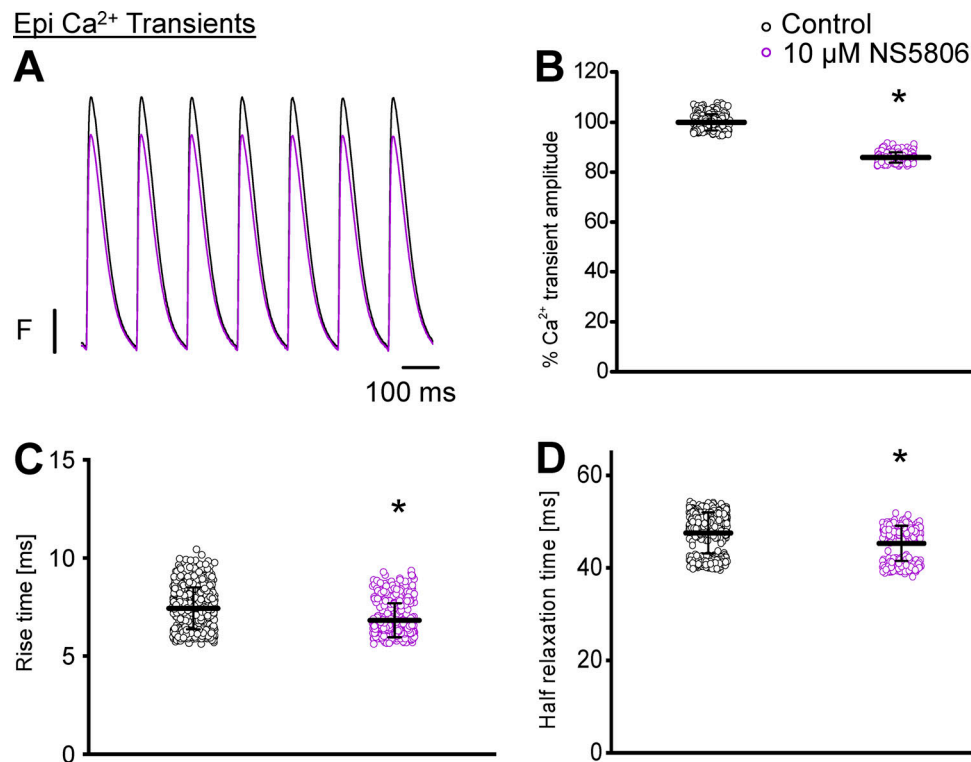
Figure 11. NS5806 decreases the left ventricle developed pressure by decreasing the amplitude and the duration of Ca 2+ transients. (A) Effect of 10 \mu M NS5806 on the time course of epicardial Ca 2+ transients. (B) The significant effect (*, P < 0.001 ) on the amplitude ( 100.1 \pm 3.2\% , 179 measurements for the control, black circles vs. 85.9 \pm 2.1\% , 180 measurements for NS5806, violet circles). (C) 10 \mu M NS5806 has a significant effect (*, P < 0.01 ) on the rise time of epicardial Ca 2+ transients ( 7.42 \pm 1.06 ms, 604 measurements for the control, black circles vs. 6.8 \pm 0.8 ms, 480 measurements for NS5806, violet circles). (D) 10 \mu M NS5806 has a significant effect (*, P < 0.01 ) on the half relaxation time of epicardial Ca 2+ transients ( 47.5 \pm 4.4 ms, 594 measurements for the control, black circles vs. 45.1 \pm 3.8 ms, 480 measurements for NS5806, violet circles). n = 4 hearts.
