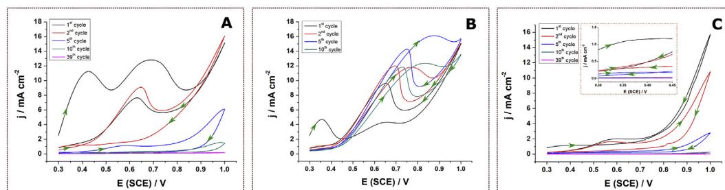
Figure 6. Voltamperometric cycles made at 50 \text{ mVs}^{-1} with Cu electrodes in A) O. vulgare , B) O. x apilii and C) T. vulgare essential oils in hydroalcoholic solution (inset correspond to record detail in region between 0.30 and 0.45 V).
