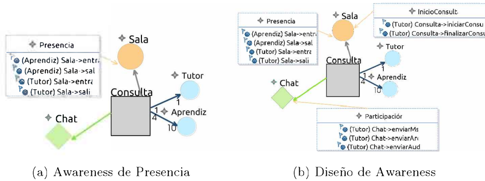
Figura 6: Modelado de Awareness
