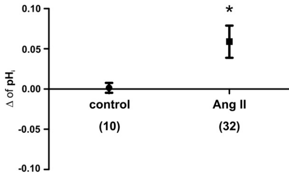
Fig. 4. Ang II (100 nmol/L) induced a slight but significant alkalization of isolated cardiomyocytes. Since intracellular pH ( pH_i ) recordings were performed in nominally absence of bicarbonate in the medium (Krebs-Hepes buffer) the rise in pH_i should be attributed to an enhanced activity of the NHE-1 in the presence of Ang II. Numbers between brackets denote the number of cardiomyocytes per experimental group. * means P < 0.05 ; t-test.
