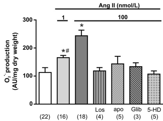
Fig. 6. Ang II dose-dependently increased myocardial superoxide ( O_2^{\cdot -} ) production. The effect of 100 nmol/L Ang II was further explored detecting that it was completely canceled by AT1 receptor blockade with losartan (Los), NOX inhibition with apocynin (apo) and mK_{ATP} channel blockade with either glibenclamide (Glib) or 5-HD. Numbers between brackets denote the number of experiments per group. * means P < 0.05 vs. control, # means P < 0.05 vs. 100 nmol/L Ang; ANOVA.
