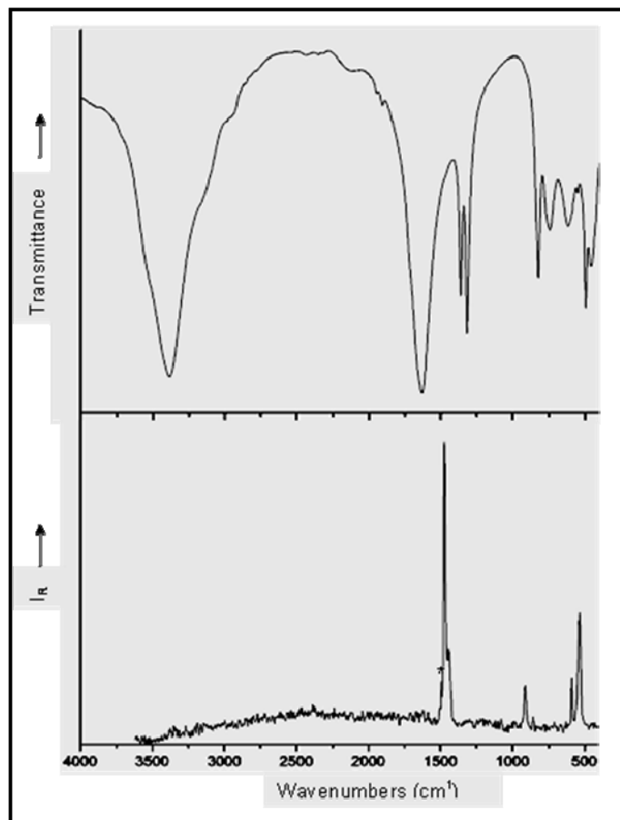
Figure 2. FTIR (above) and FT-Raman spectra (below) of \alpha\text{-ZnC}_2\text{O}_4\cdot 2\text{H}_2\text{O} in the spectral range between 4000 and 400 \text{cm}^{-1} (*this band (1492 \text{cm}^{-1} )) originates in an instrumental noise).
