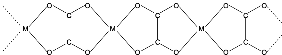
Figure 1. Schematic drawing of the infinite chain arrangement present in M^{II} -oxalates of composition M^{II}C_2O_4 \cdot 2H_2O .
