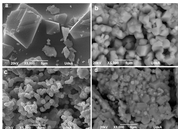
Figure 3 SEM images of spinel materials obtained by solid state: (a) \text{LiMn}_2\text{O}_4 and (b) \text{LiNi}_{0.5}\text{Mn}_{1.5}\text{O}_4 . Sol-gel: (c) \text{LiMn}_2\text{O}_4 and (d) \text{LiNi}_{0.5}\text{Mn}_{1.5}\text{O}_4
