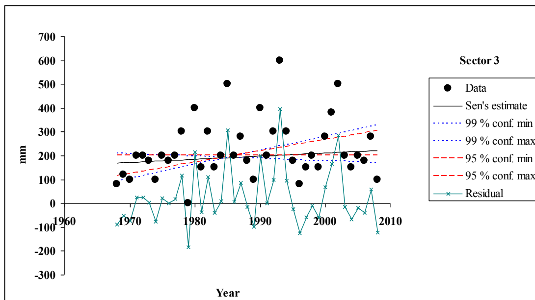
Figure 7. Trend statistics of annual soil water surplus (sws) using the Mann-Kendall test and Sen’s slope.
