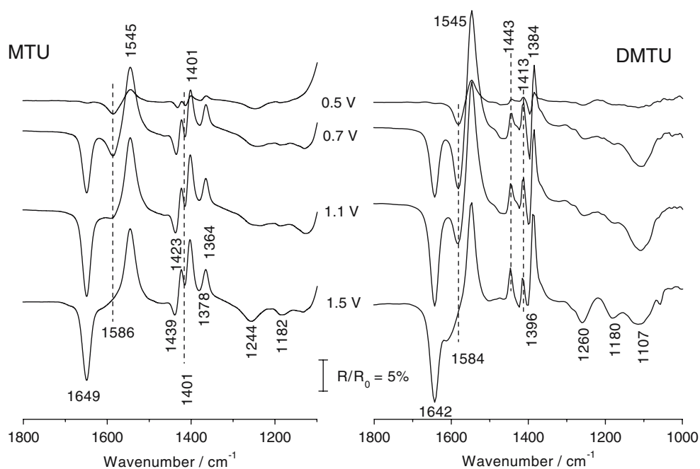
Fig. 6 p -Polarised FTIRRAS spectra of 0.1 M MTU and 0.1 M DMTU on gold in 0.1 M sulphuric acid deuterium oxide at different sampling potentials. E_{\text{ref}}=0.05 V
