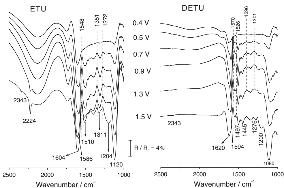
Fig. 7 p -Polarised FTIRRAS spectra of 0.1 M ETU and 0.1 M DETU on gold in aqueous 0.1 M perchloric acid at different sampling potentials. E_{\text{ref}}=0.05 V
