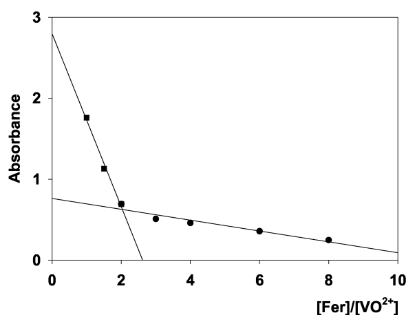
Fig. 2. Spectrophotometric titration of VO 2+ with ferulic acid at pH 7.0 for λ = 790 nm.
