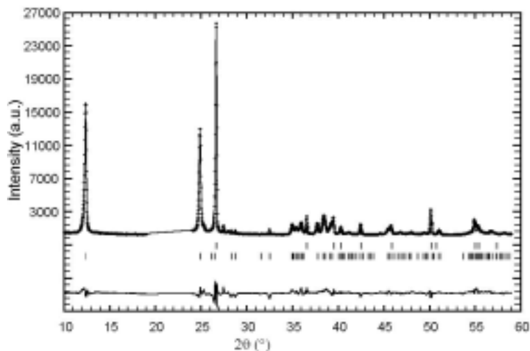
FIG. 2. Observed (dotted line) and calculated (solid line) diffraction patterns for a 70/30 kaolinite-quartz standard sample. The region between 20 and 24° 2\theta was excluded. ( R_{wp}=30.2 , R_{exp}=4.6 ).
