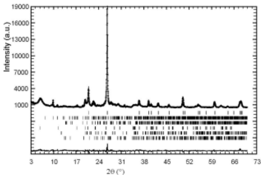
FIG. 7. Observed (dotted line) and calculated (solid line) diffraction patterns for zeolitized tuff A40, Cerro Barcino Formation ( R_{wp}=16.3 , R_{exp}=8.1 ).
