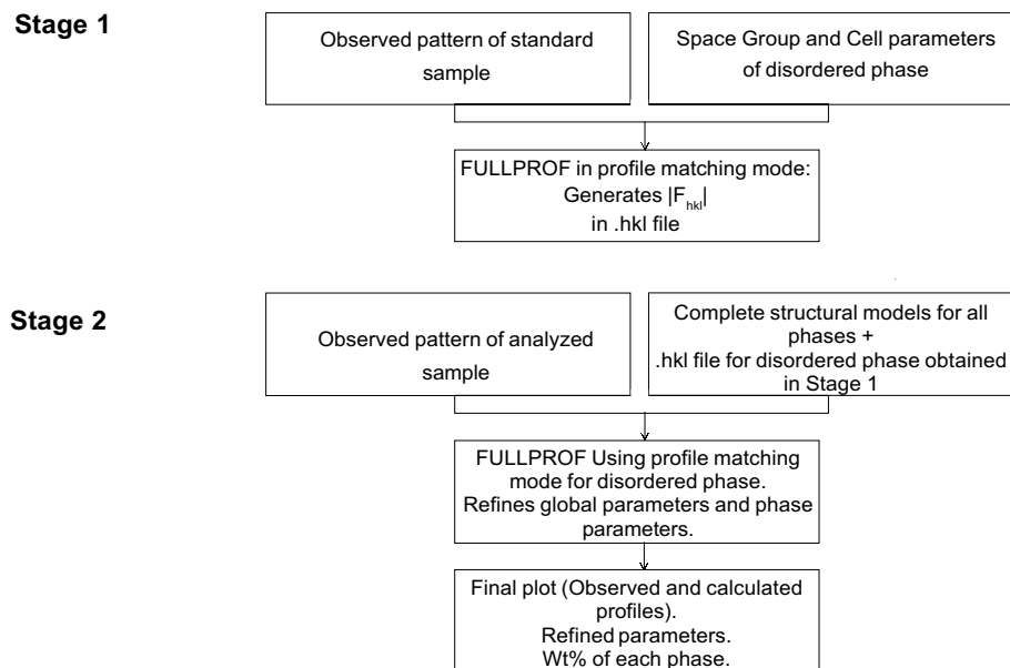
FIG. 1. Flow diagram for quantitative phase analysis with FULLPROF, including a phase in profile matching mode.
