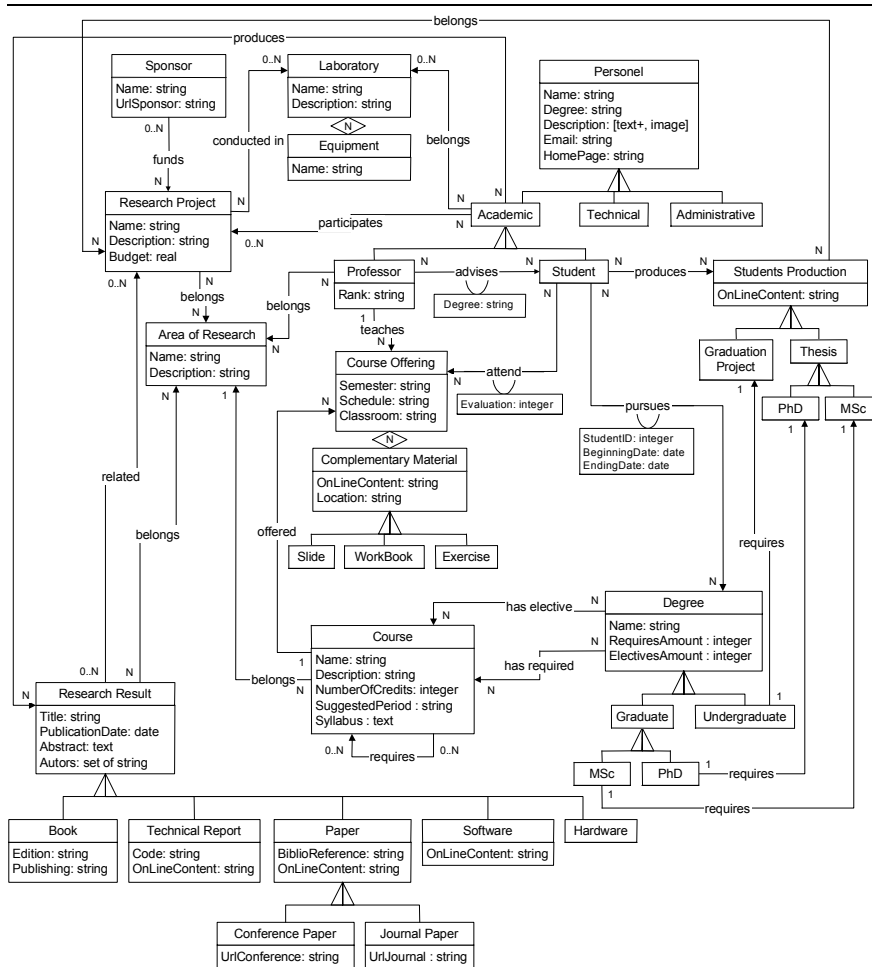
Fig. 1. Conceptual Schema of the Academic Department Site.
