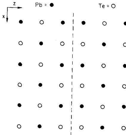
Fig. 1. Two-dimensional view of the PbTe system with a domain wall (dotted line) on the (001) axis. Note that the phase to the right of the wall can be obtained from the phase to the left by a lattice displacement of half a unit.
