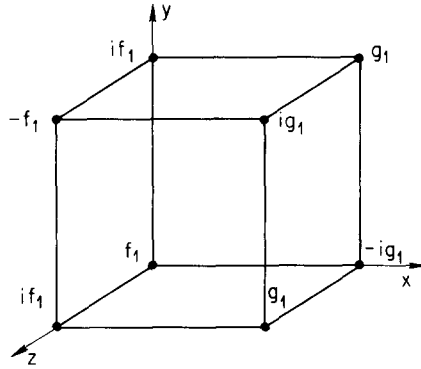
Fig. 4. Lattice wave function of the modes localized over the wall.
