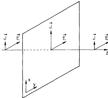
Fig. 2. An external electric field E along the wall induces a current J perpendicular to E . The current decreases away from the wall because the wave function is exponentially small at |z| \gg 1 .
