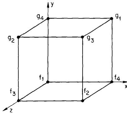
Fig. 3. Redefinition of the field \psi in a unit cell.
