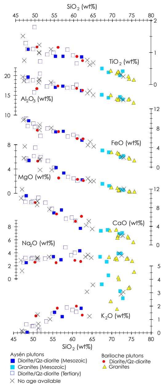
Figure 3. Silica variation diagrams (Harker) showing the trend of representative samples from the North Patagonian batholith in the regions of Aysén and Bariloche. Qz—quartz.
