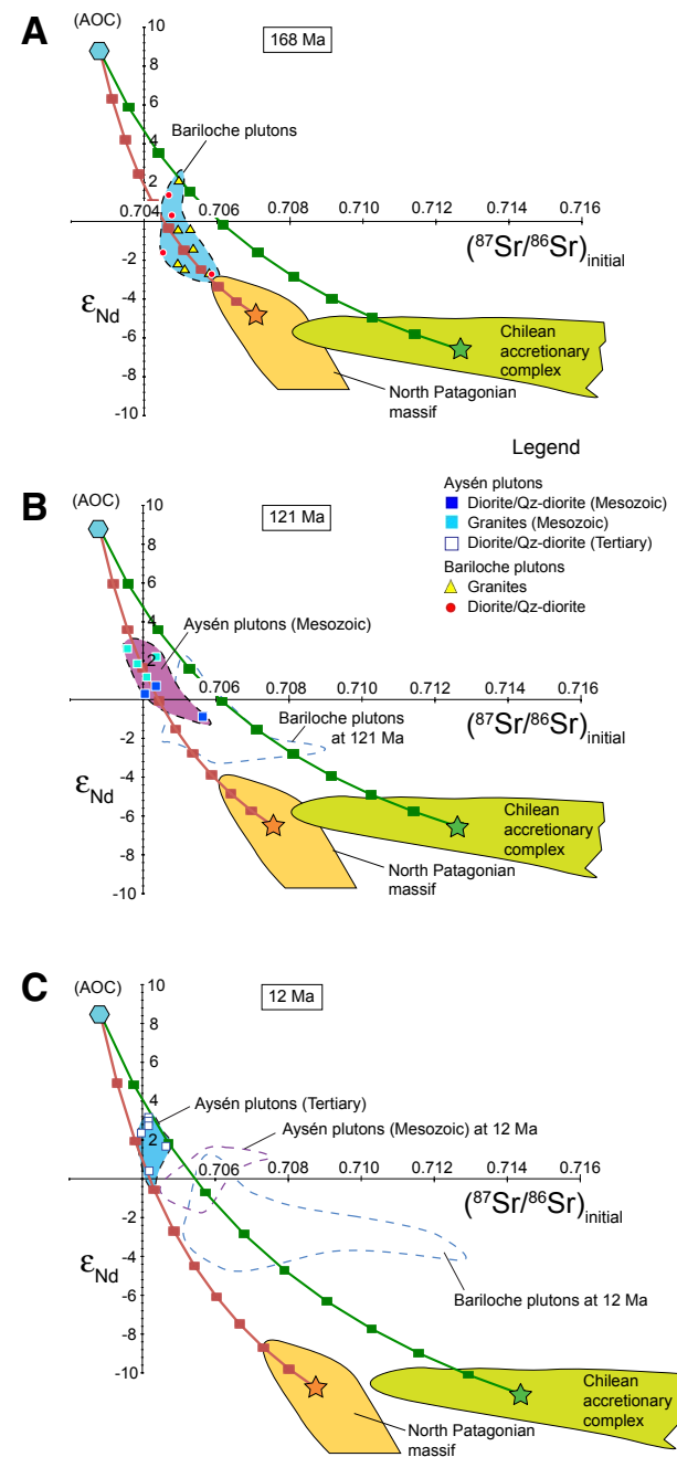
Figure 11. (A–C) Mixing models of initial isotopic ratios of Sr and Nd (Nd in epsilon notation), showing possible mélangé source compositions using a juvenile end member, represented by the altered oceanic crust (AOC), and two evolved end members, represented by the North Patagonian massif and the Chilean accretionary complex. These are compared with isotopic ratios of plutons normalized to the three peaks of plutonic activity at 168, 121, and 12 Ma. Squares along the mixing lines represent 10% increments of end members involved. Qz—quartz.
