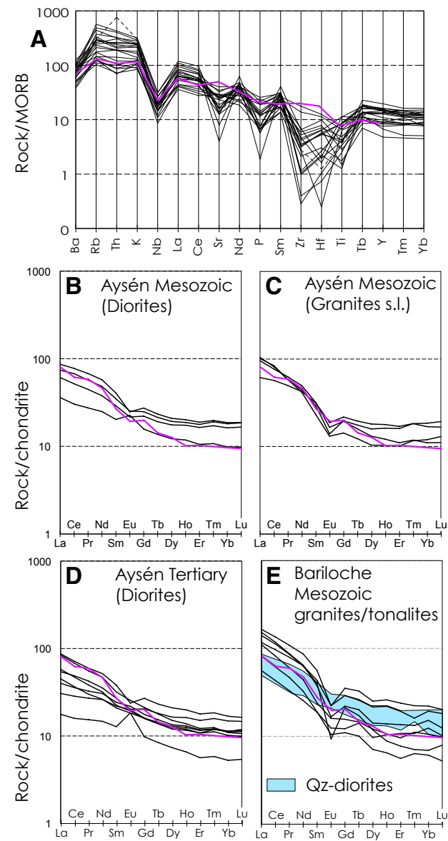
Figure 4. Trace-element diagrams of samples from the North Patagonian batholith. (A) Mid-ocean-ridge basalt (MORB)-normalized (Thompson et al., 1984) spider diagram. (B–E) Chondrite-normalized (Nakamura, 1974) plots of rare earth elements (REEs) comparing patterns of dioritic and granitic rocks from the Bariloche and Aysén regions. In all diagrams, the average composition of continental andesites (Kelemen et al., 2003) is shown (purple line). Qz—quartz.
