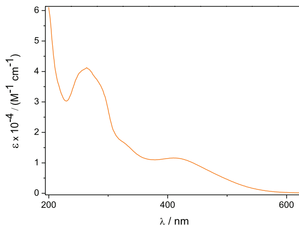
Figure 1. UV-Vis spectrum of 1 in \text{H}_2\text{O} at room temperature.
