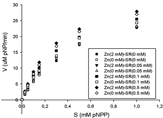
Fig. 4 Effects of Zn 2+ and SR on kinetics of ALP-catalyzed hydrolysis of pNPP. The initial rates of hydrolysis of increasing concentrations of pNPP in the presence of 0 mM Zn 2+ (white symbols) or 2 mM Zn 2+ (black symbols) and different concentrations of SR were determined
