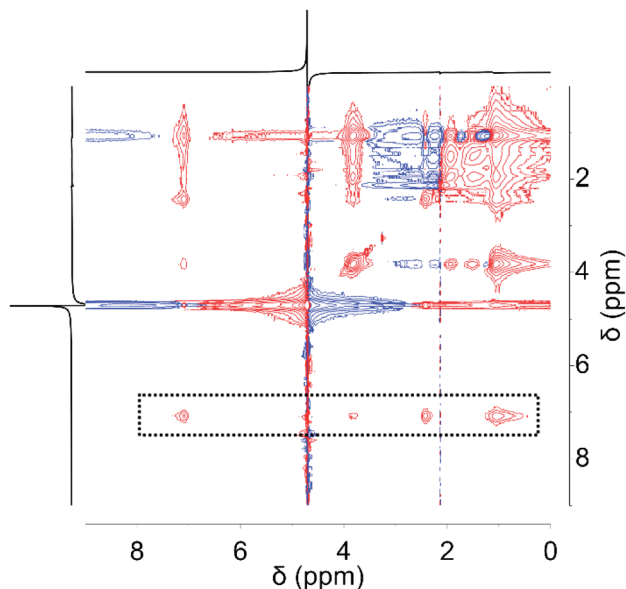
Fig. 3 Nuclear Overhauser effect spectroscopy (NOESY) analysis for ZIF-8@microgel composite material. Dashed area marks features arising from coupling between imidazole and microgel signals.
