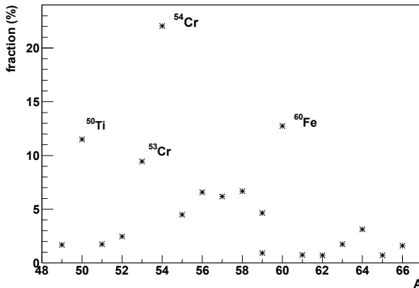
Fig. 1. Most abundant elements produced in a strange star-strange star merger.
