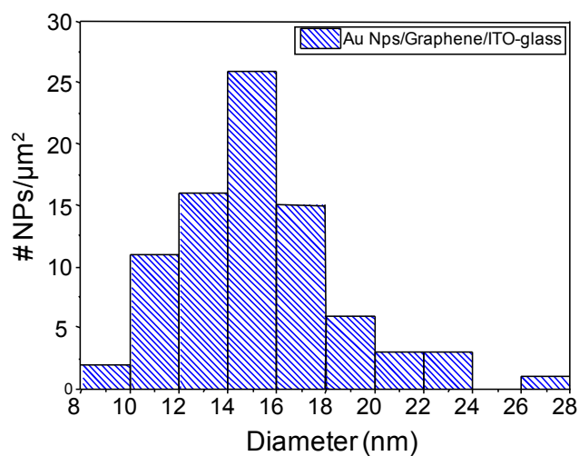
Figure S2. SEM image and its corresponding histogram which exhibit the # of Au NPs/ \mu\text{m}^2 counted in a selected “low agglomerated area” on graphene.
