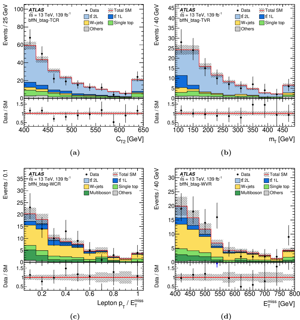
Figure 9. Selected kinematic distributions in bffN_btag CRs and VRs: (a) C_{T2} in the TCR, (b) m_T in the TVR, (c) p_T^{\ell}/E_T^{\text{miss}} in the WCR, (d) E_T^{\text{miss}} in the WVR. The distributions shown are post-fit, i.e. each background is scaled by a normalisation factor obtained from a background-only likelihood fit to the CRs (see table 14). The hatched area around the total SM prediction and the hatched band in the Data/SM ratio include all statistical and systematic uncertainties. The last (first) bin contains overflows (underflows).
