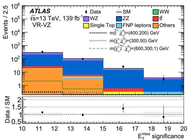
(e) E_T^{\text{miss}} significance distribution in VR-VZ
