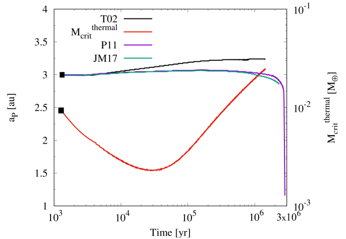
Fig. 8. Time evolution of the semi-major axis of the planet for the simulations corresponding to the case where the hybrid accretion of pebbles and planetesimals is considered. The black line corresponds to the fiducial simulation where type I migration recipes from Tanaka et al. (2002) are adopted. The purple and green lines correspond to the cases where type I migration recipes from Paardekooper et al. (2011) and Jiménez & Masset (2017) are considered, respectively. For the cases T02 and JM17, the planet remains in a migration trap until it opens a gap in the gas disk. The red line represents the values of the critical thermal mass associated to the thermal torque (for the T02 case). As this mass is always much lower than the mass of the planet, the thermal torque does not play any effect in the torque over the planet.
