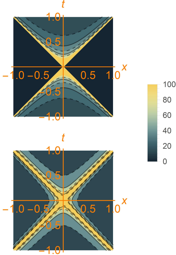
FIG. 1. Contour plot of the invariant space time density (45) (top) and the Dirac density (46) (bottom), for m \equiv mc/\hbar = 1 . The first one vanishes in the spacelike region (here x and t \equiv ct are in units of \hbar/mc ).
