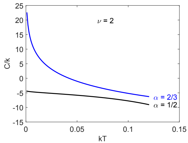
Figure 2: Two dimensions: specific heats at the two poles versus temperature T .
