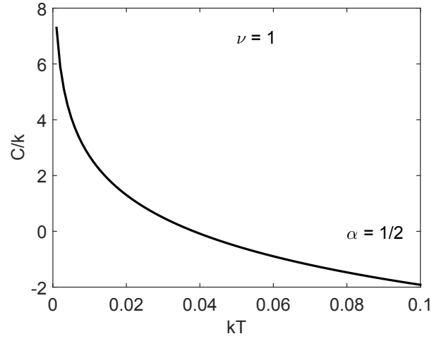
Figure 1: One dimension: specific heats at the pole versus temperature T .
