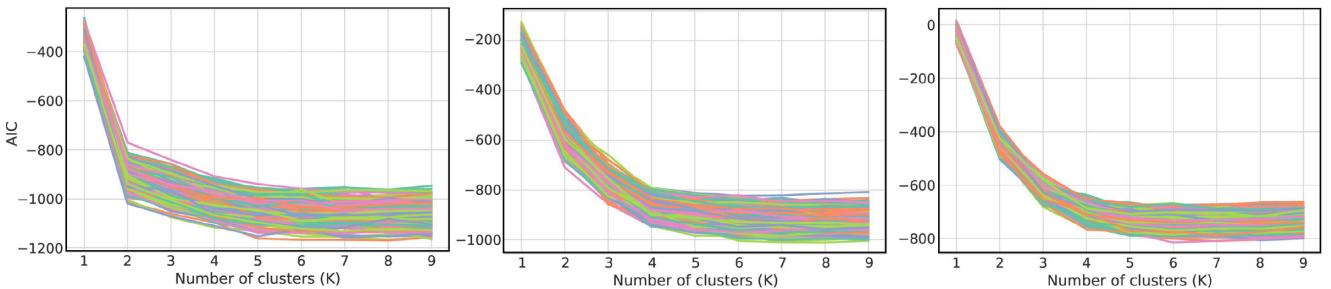
Figure 11. AIC as a function of the number of the fitted Gaussian components ( K ) obtained for the 500 experiments performed considering the simulated case of two groups of objects (left-hand panel), four groups (central panel), and considering a sample of objects following a uniform distribution in colours (g' - z') and (g' - i') (right-hand panel).
