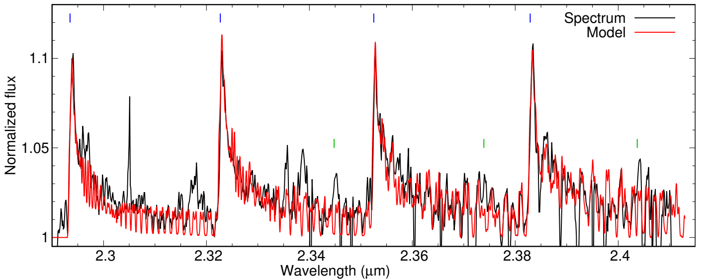
Fig. 3. Portion of the K-band spectrum of 12 Vul with ^{12}\text{CO} emission (black). The synthetic spectrum is plotted in red. Blue and green tics point out the position of the ^{12}\text{CO} and ^{13}\text{CO} band heads, respectively.
