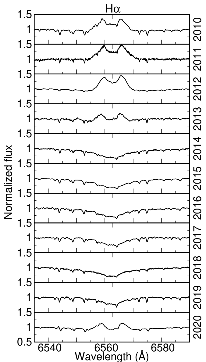
Fig. 1. Optical spectra of 12 Vul around the \text{H}\alpha line region. The \text{H}\alpha line profile was in emission between 2010 and 2013. Between 2014 and 2019, there was no evidence of emission superimposed to the photospheric absorption. In 2020, the line profile was again in emission.
