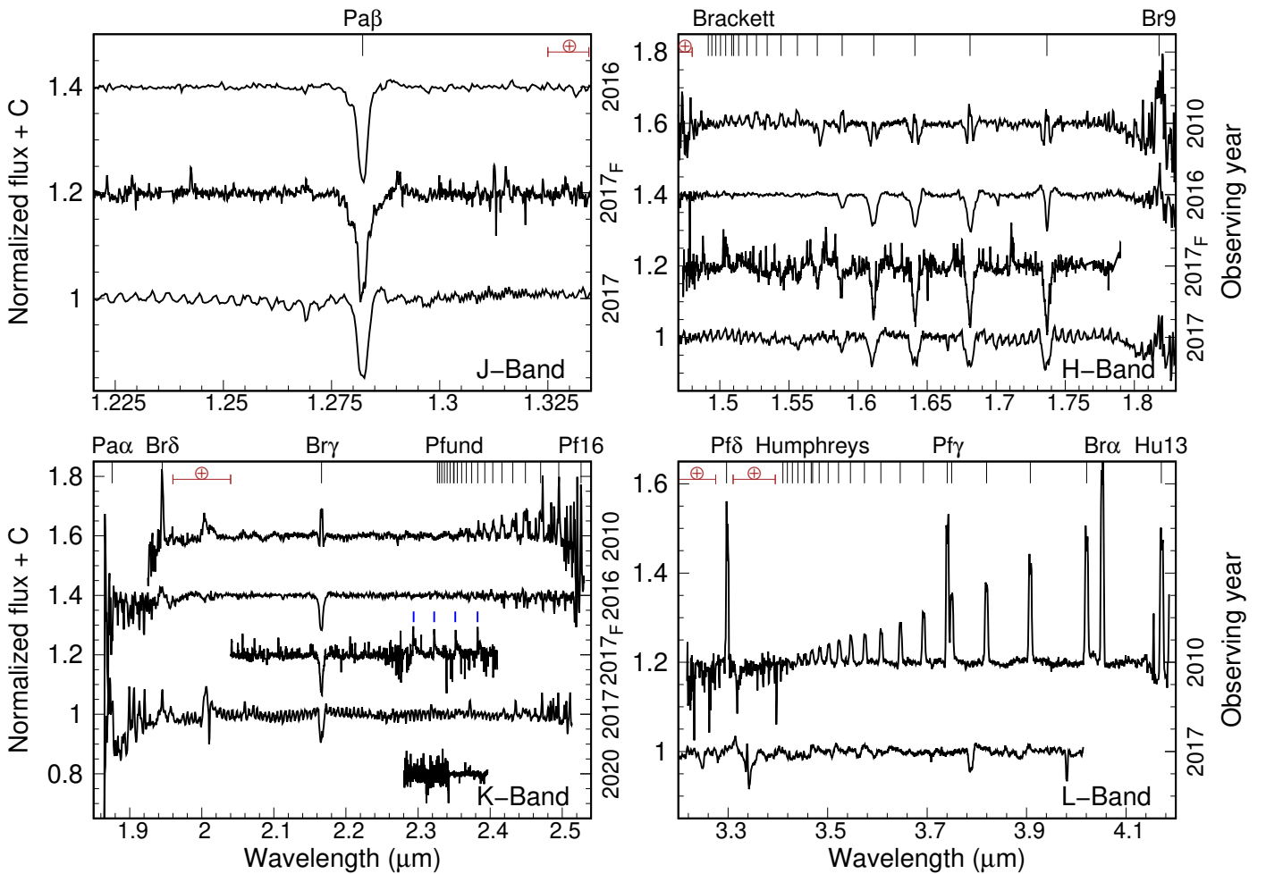
Fig. 2. NIR spectra of 12 Vul in the J- (upper-left panel), H- (upper-right panel), K- (lower-left panel), and L-bands (lower-right panel). All the spectra were taken with GNIRS, except the one obtained with FIRE, which is pointed to with an F in the observing year. Spectra were normalized and vertically shifted for a better visualization. Positions of the hydrogen lines are marked in the top of each panel, and spectral ranges with telluric remnants are pointed out with the symbol \oplus . The ^{12}\text{CO} band heads in emission in the K-band are indicated with blue tics.
