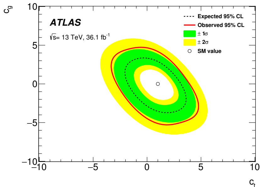
Figure 15. Observed (solid) and expected (dashed) exclusion limits at 95% CL in the c_g versus c_t plane for modified t\bar{t}H and ggH couplings. The uncertainties in the expected limit corresponding to one and two standard deviations are displayed as green and yellow bands respectively. The hollow circle denotes the tree-level SM values of the parameters: c_g = 0 and c_t = 1 .
