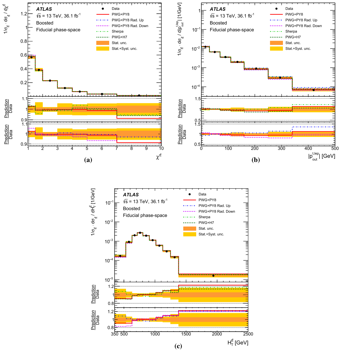
Fig. 41 Particle-level normalised differential cross-sections as a function of a \chi^{\text{if}} , b |p_{\text{out}}^{\text{t,lep}}| and c H_T^{\text{if}} in the boosted topology, compared with different Monte Carlo predictions. The bands represent the statisti-
