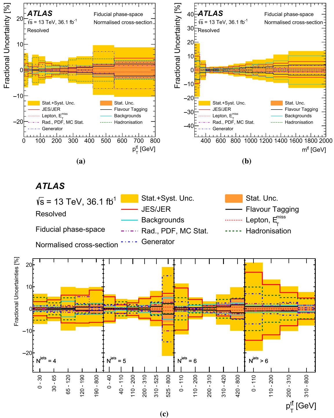
Fig. 18 Uncertainties in the particle-level normalised differential cross-sections as a function of a the transverse momentum, b the mass of the t\bar{t} system, and c the transverse momentum of the t\bar{t} system as
