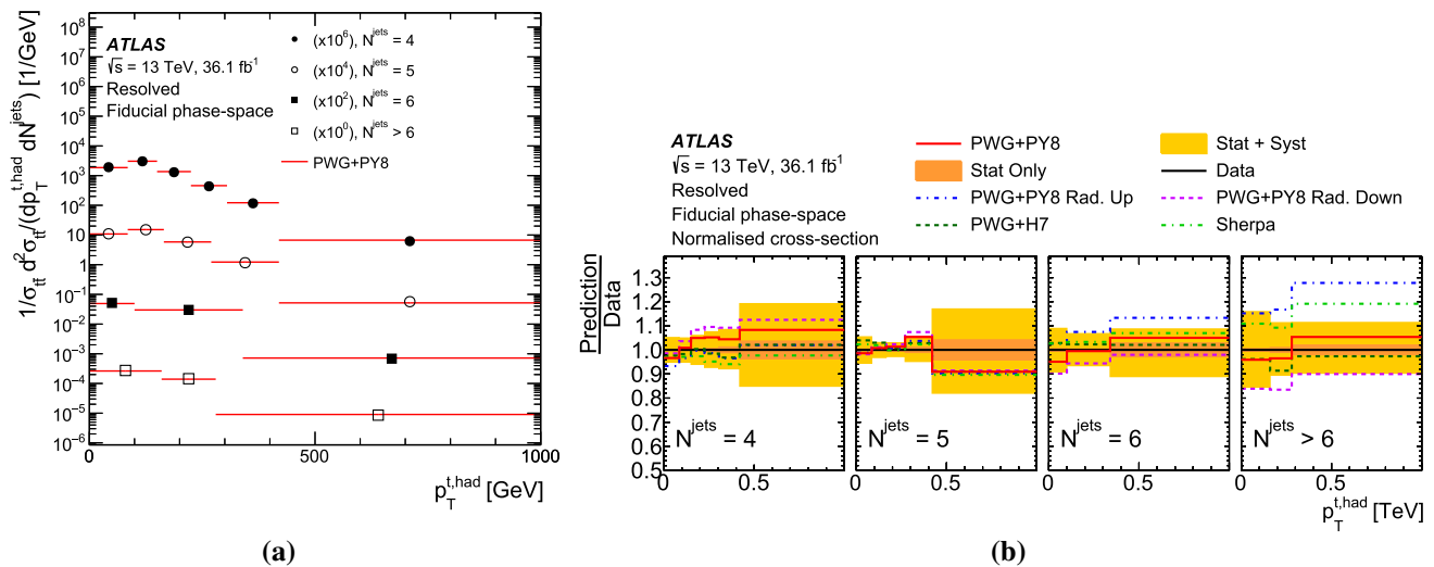
Fig. 29 a Particle-level normalised differential cross-section as a function of p_T^{t, \text{had}} in bins of the jet multiplicity in the resolved topology compared with the prediction obtained with the POWHEG+PYTHIA8 MC
