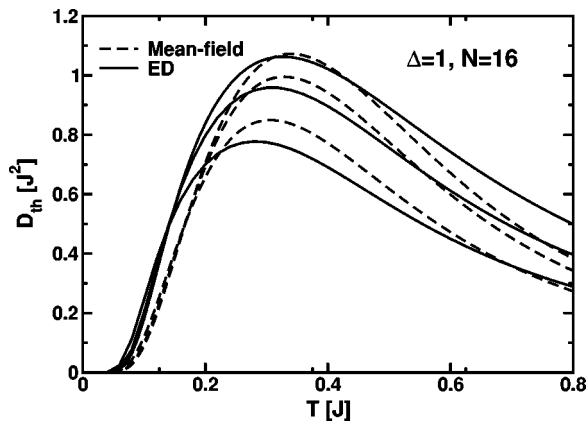
FIG. 4. Comparison between exact diagonalization (solid lines) and mean-field approximation (dashed lines) on finite systems with N=16 sites for various values of \alpha=0, 0.05, 0.15 (top to bottom) and \Delta=1 .
