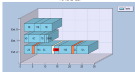
Fig.9 (c). Resulting schedule after a RightMove. TT=49.73 h.
