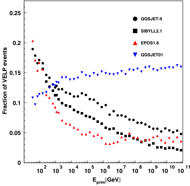
FIG. 4 (color online). Fraction of VELP events versus primary energy for the case of proton-nitrogen collisions.
