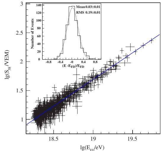
FIG. 1 (color online). Correlation between \lg S_{38^\circ} and \lg E_{FD} for the 661 hybrid events used in the fit. The full line is the best fit to the data. The fractional differences between the two energy estimators are inset.
