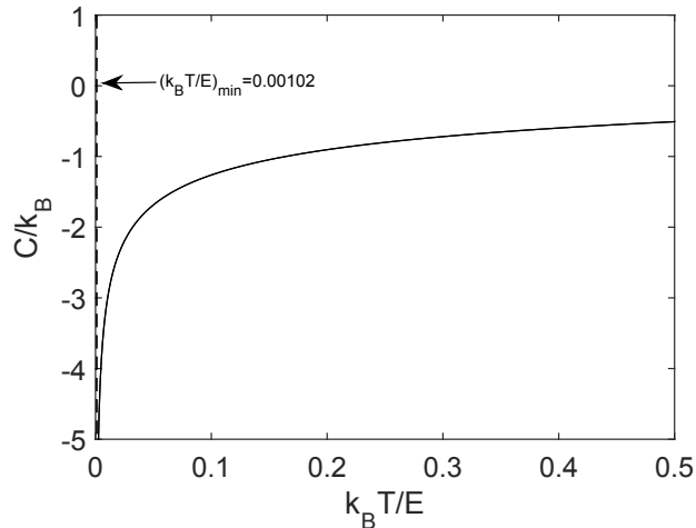
Figure 2: Specific heat versus k_B T/E for q = 1/3 . It is well known that gravitational effects make specific heats to be negative [81]. This is clearly appreciated here.
