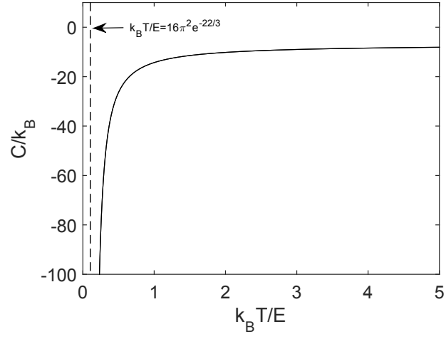
Figure 1: Specific heat versus k_B T/E for q = 3/2 . It is well known that gravitational effects make specific heats to be negative [81]. This is clearly appreciated in this graph and in the following one.
