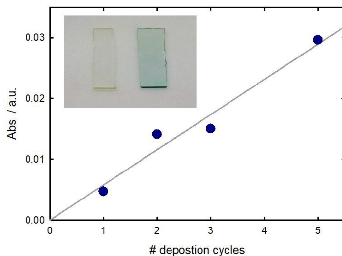
Figure 4. Absorbance at 680 nm of LbL-modified glass substrates as a function of the number of deposition cycles. Inset: digital images of the glass plate before and after 5 cycles of deposition.
