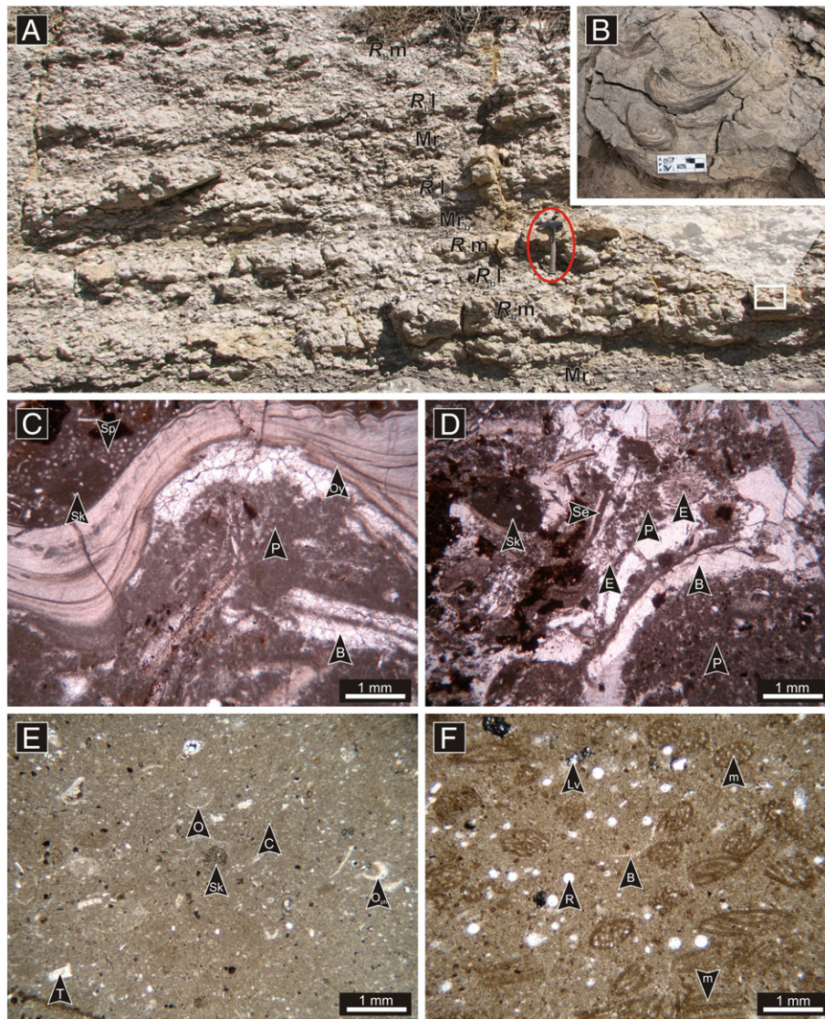
Fig. 6. A) Field exposure of facies association 1 (oyster auto-parabiostrome dominated middle ramp), lower Valanginian, Cara Cura (see hammer for scale and lithofacies code in Table 1). B) Detail of oysters ( Aetostreon latissimum Lamarck) in bioclastic floatstone/rudstones ( R_b , F_b , m ). C–D) Thin sections of bioclastic floatstone/rudstones ( R_b , F_b , m ), showing a peloidal matrix and fragmented skeletal particles. E–F) Thin sections of laminated wackestones ( W_b , h ). References: (B) recrystallized bivalves, (C) calcisphaeres and/or calpionellids, (E) echinoderms, (Lv) volcanic clasts, (m) crustacean microcoprolites, (O) ostracods, ( O_{pi} ) ophiurids, (Oy) oysters, (P) peloids, (R) radiolarians, (Se) serpulid fragments, (Sk) steinkerns (internal molds of gastropods), (Sp) sponge spicules, (T) terrigenes.
