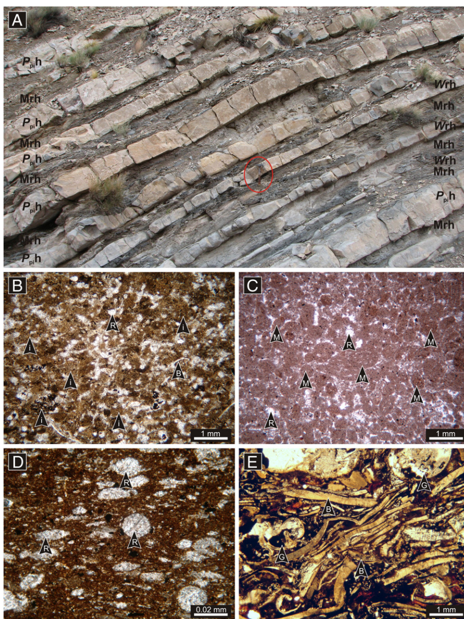
Fig. 9. A) Field exposure of facies association 4 (proximal outer ramp), upper Tithonian, Arroyo Loncoche section (see lithofacies code in Table 1). B) Intraclastic packstones ( P_h ) showing abundant rounded to angular micritic intraclasts. C) Peloidal packstones ( P_{pih} ) consisting of crustacean microcoprolite accumulations. D) Radiolaritic wackestones ( W_rh ) showing abundant spumellarid and nassellarid radiolaria. E) Bioclastic rudstones ( Rf_b ) containing abundant bivalve fragments and gastropods. References: (B) bivalves, (G) gastropods, (i) intraclasts, (M) crustacean microcoprolites ( Palaxius caracaraensis Kietzmann), (R) radiolarians.
