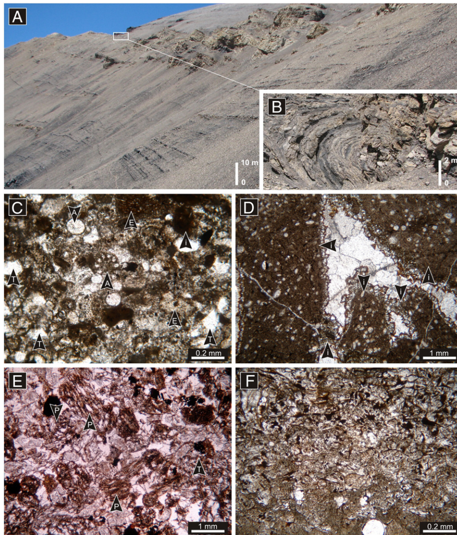
Fig. 12. A–B) Field exposure of facies association 7 (carbonate slope), upper Tithonian–lower Berriasian, Cerro Domuyo section, showing slumped fine grained intervals and lenticular sandy packstones ( P_{bi,m} , P_{bi,h} ). C) Sandy bioclastic packstones ( P_{bi,m} , P_{bi,h} ) in lenticular sandy interval. D) Intraclastic breccia ( B_i ) consisting of radiolaritic wackestone intraclasts. E) Lapillite deposits ( L_m , L_g ) of coarse sand to granule grain size. F) Inverse graded tuff deposits ( T_g ) consisting of shards and pumiceous fragments. References: (A) dasycladacean algae, (E) echi-noderm fragments, (i) intraclasts, (P) pumiceous fragments, (T) terrigenes.
