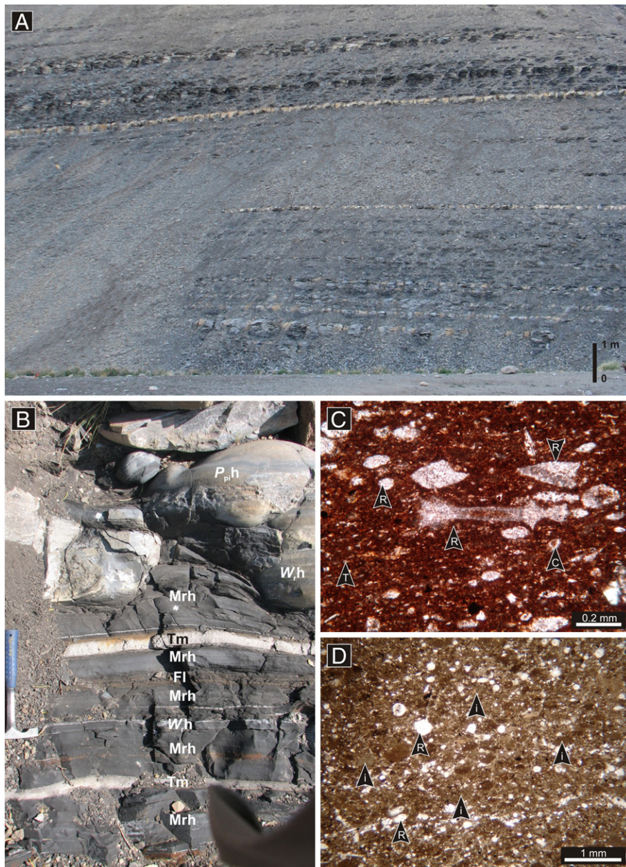
Fig. 11. A) Field exposure of facies association 6 (distal outer ramp to basin), Berriasian, Arroyo Rahue section, showing the alternation of marls with intraclastic packstones (P pi h) and radiolaritic wackestones (W h ). B) Detail of facies association 6, lower Tithonian, Cañada Ancha section, showing alternation of marls (Mrh), laminated wackestones (W h ) and pyroclastic deposits (T m , T g ) (see lithofacies code in Table 1). C) Radiolaritic wackestones (W h ) showing abundant radiolarians and terrigenes. D) Normal graded intraclastic packstone (P pi h) composed by micritic intraclasts and radiolarians. References: (C) calpionellids, (i) intraclasts, (R) radiolarians, (T) terrigenes.
