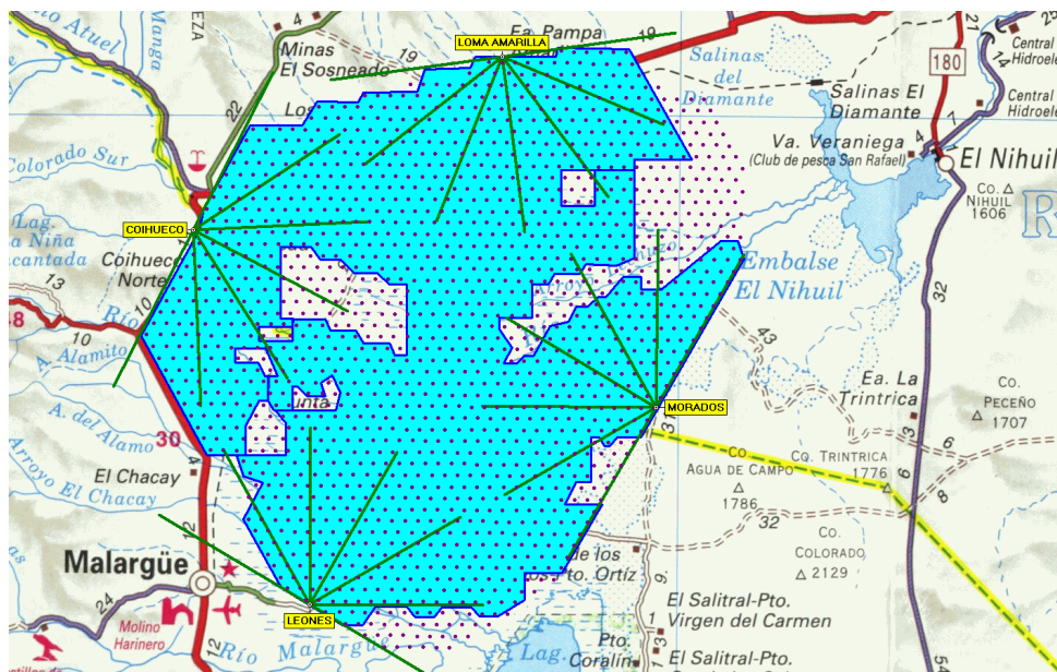
Figure 1: Layout of the Pierre Auger Southern Observatory. The dots represent the position of each of the 1600 SD stations. The 1430 SD stations deployed and activated as of 30 September 2007 lie in the area shaded blue. The 4 FD sites are labeled in yellow, with green lines indicating the field of view of the six telescopes at each site. To give the scale of the Observatory, the lengths of the green line correspond to 20 km.
