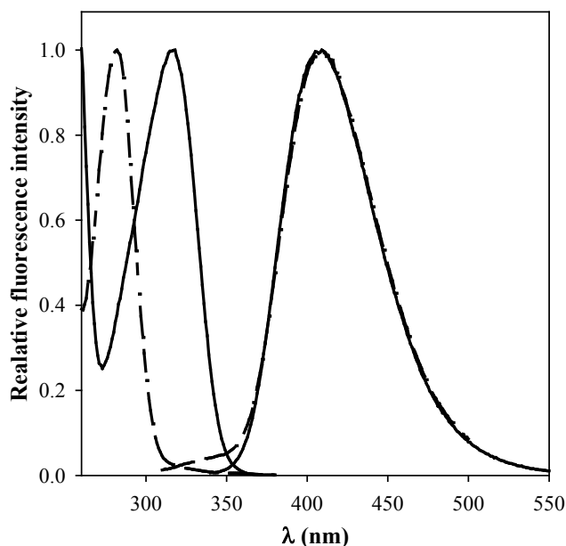
Figure 8. Normalized emission and excitation spectra of Tyr 2 in acid (dashed line) and alkaline (solid line) aqueous solutions. Emission spectra in acid and alkaline solution were obtained upon excitation at 280 and 315 nm, respectively. Excitation spectrum was obtained at 410 nm.
