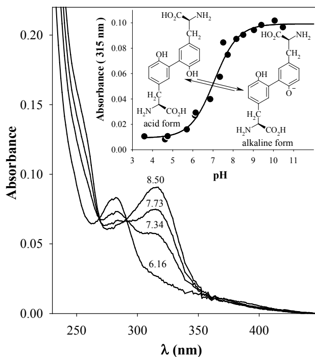
Figure 7. Absorption spectra of air equilibrated aqueous solution of purified Tyr 2 at different pH values. The pH values appear above each spectrum. Inset: acid-base equilibrium in aqueous solution of Tyr 2 and the variation of the absorbance at 315 nm (circles) as a function of pH; the solid line represents the absorbance calculated by fitting the experimental data to Equation 1. [Tyr 2 ]= 12 μM.
