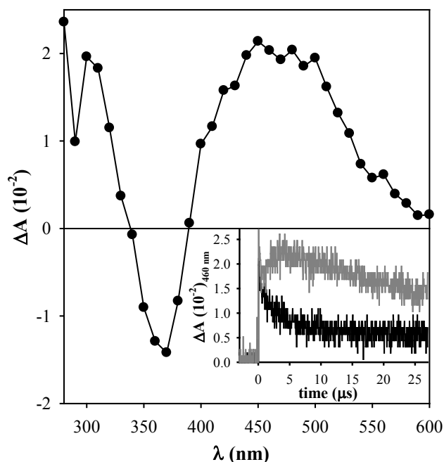
Figure 4. Transient absorption spectrum of \text{N}_2 flushed aqueous solution of Ptr ( 75 \mu\text{M} ) at pH 5 in the presence of 1 mM DABCO ( 5.4 \mu\text{s} after the laser pulse). Inset: Time dependence of the absorbance at 460 nm at 0 (black line) and 1 mM (gray line) of DABCO.
