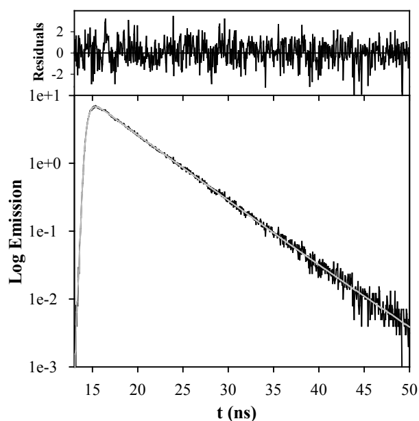
Figure 9. Fluorescence decays and monoexponential fitting analysis of the Tyr 2 emission in alkaline aqueous solution (17 \mu M, pH = 9.75, \lambda_{exc} = 341 nm, \lambda_{an} = 410 nm).
