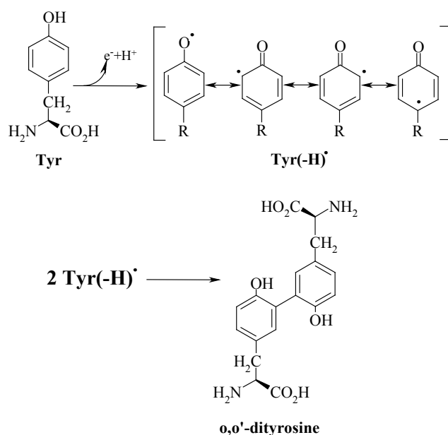
Figure 1. Postulated oxidative formation of dimer o,o'-dityrosine (Tyr 2 ).
