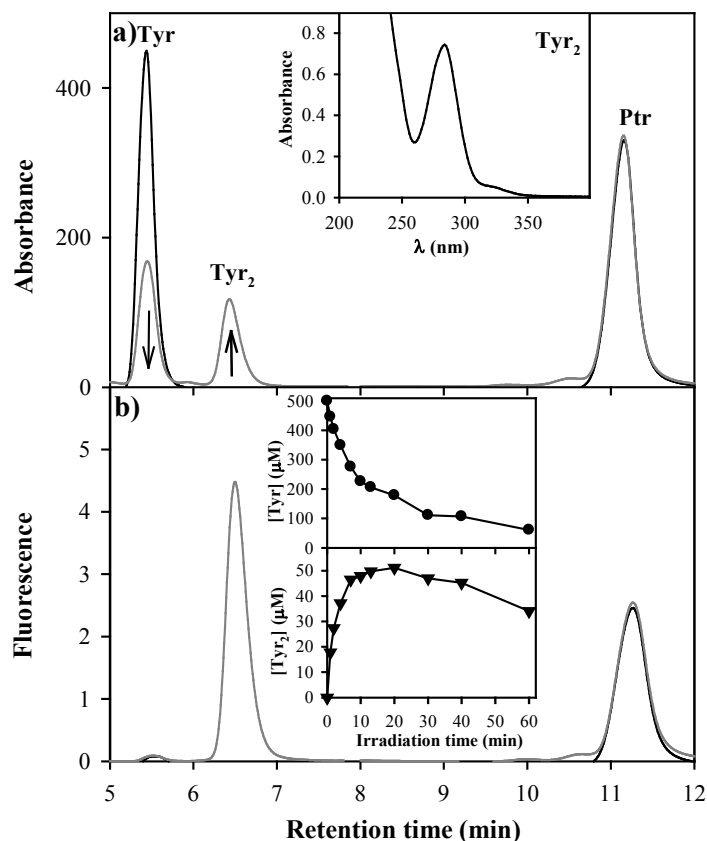
Figure 5. Chromatograms, obtained using a) the HPLC1-PDA detector at 280 nm and b) HPLC1-FL detector (excitation at 280 nm, emission at 410 nm), of a solution containing Tyr and Ptr before (black line) and after 10 min (gray line) of irradiation. Inset: a) absorption spectrum of Tyr 2 in NH 4 Ac (1mM, pH= 6.0) obtained for the peak at 6.45 min in the chromatogram; b) evolution of the Tyr and Tyr 2 concentration as a function of irradiation time. [Ptr] 0 = 100μM, [Tyr] 0 = 500μM, pH = 6.0.
