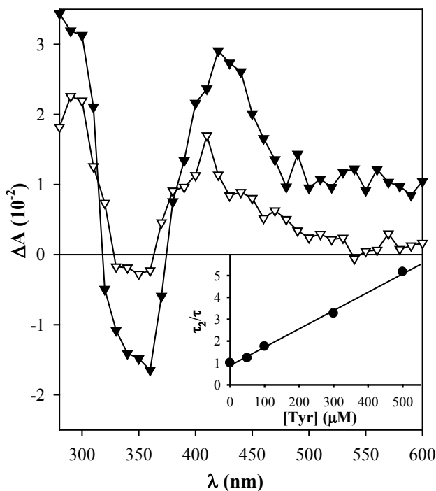
Figure 3. Transient absorption spectra of \text{N}_2 flushed aqueous solution of Ptr ( 75 \mu\text{M} ) at pH 5 in the absence (black triangle, 0.4 \mu\text{s} after the laser pulse) or in the presence of 500 \mu\text{M} Tyr (white triangle, 15 \mu\text{s} after the laser pulse). Inset: corresponding Stern-Volmer plot.
