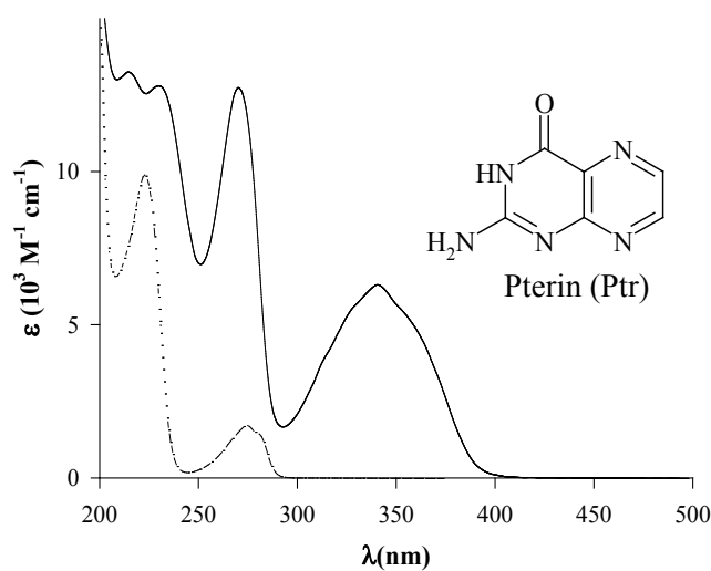
Figure 2. Absorption spectra of pterin (Ptr, solid line) and tyrosine (Tyr, dashed line) in air-equilibrated aqueous solutions at pH 5.5. Inset: molecular structure of Ptr.
