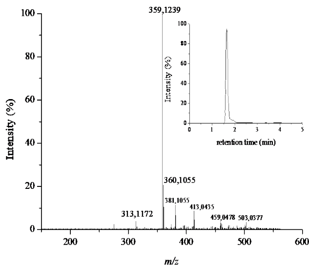
Figure 6. Mass spectrum obtained from UPLC-QToF-MS analysis of an isolated aqueous solution of Tyr 2 (14 \mu M). Inset: Mass chromatogram of m/z 359.1239 Da. Mode ESI, Voltage= 30 V.
