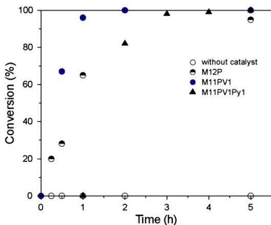
Fig. 3. Conversion vs. reaction time for the oxidation reaction of Scheme 1 : without catalyst and with M12P, M11PV1 or M11PV1Py1 as catalysts. Sulfide: 35% H 2 O 2 ; catalyst = 0.7: 2: 0.01 mmol; acetonitrile: 5 mL.
