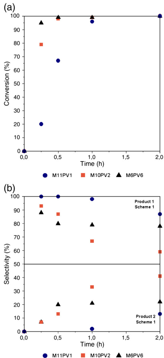
Fig. 4. a) Conversion vs. reaction time for the catalytic oxidation of Scheme 1 , using M12-xPVx as catalyst. Sulfide: 35% H 2 O 2 ; catalyst = 0.7: 2: 0.01 mmol; acetonitrile: 5 mL. b) Selectivity vs. reaction time for both products of the catalytic oxidation of Scheme 1 , using M12-xPVx as catalyst. Sulfide: 35% H 2 O 2 ; catalyst = 0.7: 2: 0.01 mmol; acetonitrile: 5 mL.
