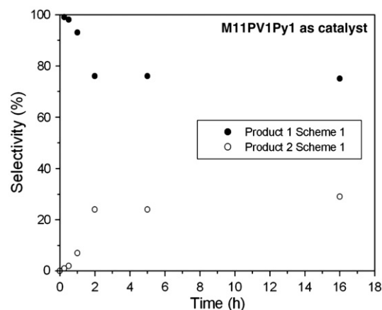
Fig. 5. Selectivity vs. reaction time for both products of the catalytic oxidation of Scheme 1 , using M11PV1Py1 as catalyst. Sulfide: 35% H 2 O 2 ; catalyst = 0.7: 2: 0.01 mmol; acetonitrile: 5 mL.
