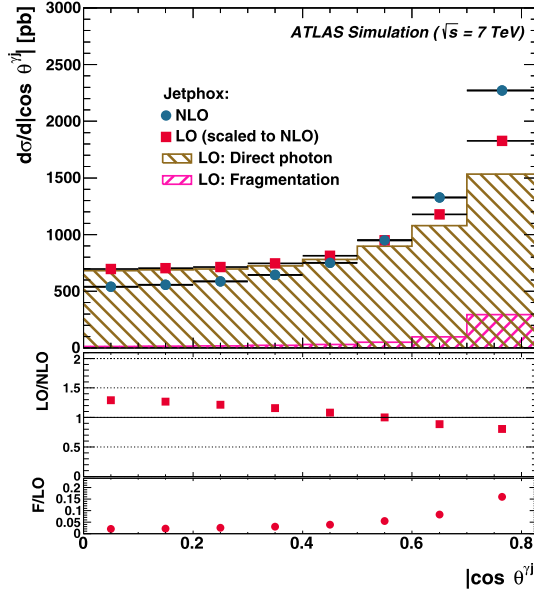
Fig. 15. The NLO QCD predicted bin-averaged cross section for isolated-photon plus jet production as a function of |\cos \theta^j| including the requirements on m^{\gamma j} and |\eta^\gamma + y^{\text{jet}}| (dots). The LO QCD calculation (squares) scaled to the NLO integrated cross section and the contributions of the direct-photon (right-hatched histogram) and fragmentation (left-hatched histogram) components are also shown. The middle part of the figure shows the ratio of the scaled LO to the NLO QCD calculations (squares); the bottom part of the figure shows the ratio of the fragmentation component to the full LO calculation (dots).
