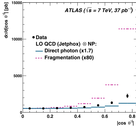
Fig. 16. The measured bin-averaged cross section for isolated-photon plus jet production (dots) as a function of |\cos \theta^j| including the requirements on m^{\gamma j} and |\eta^\gamma + y^{\text{jet}}| . The direct-photon (solid lines) and fragmentation (dashed lines) components of the LO QCD prediction are also included. The calculations were normalised to the measured cross section for |\cos \theta^j| < 0.1 ; the factors used are shown in parentheses.
