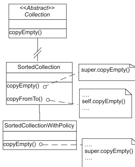
Fig. 17. Inherited and Local Invocations.
