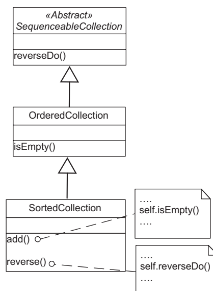
Fig. 14. Reuse of superclass behavior.
