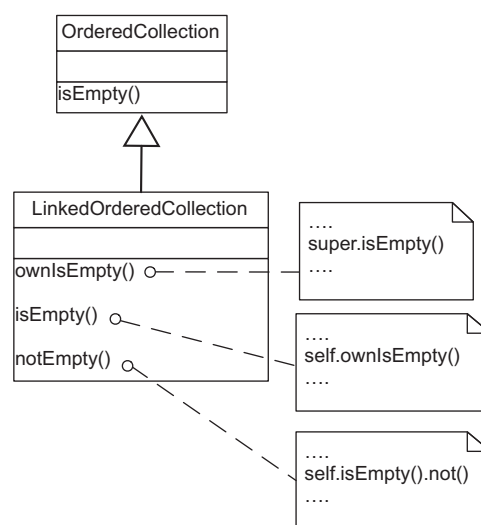
Fig. 13. Inherited and Local Invocations – Case 2.
