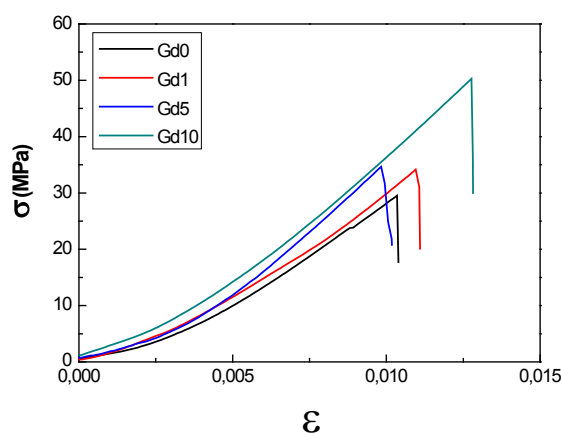
Fig. 10. Stress strain curves of the sintered bauxite Gd 2 O 3 mixtures fired at 1500 °C (examples).
