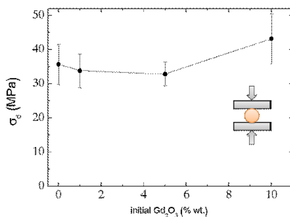
Fig. 9. Mechanical strain; diametral compression resistance of the studied samples as a function of the Gd 2 O 3 content.
