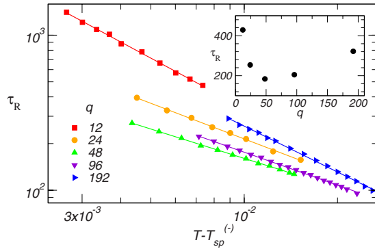
FIG. 11. Relaxation time as a function of T - T_{\text{sp}}^{(-)} for L=1000 and different values of q . Error bars are smaller than the symbol sizes. Note, however, that due to the error in the determination of T_{\text{sp}} , the points could be uniformly shifted horizontally. The continuous lines are power law fits. Inset: \tau_R as a function of q for a fixed temperature T - T_{\text{sp}} = 0.008 .
