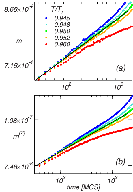
FIG. 6. Short time behavior in a supercooled state at different temperatures for q=96 and L=480 . Full lines are power law fittings for T=0.950T_t . (a) Order parameter m . (b) Second moment m^{(2)} .
