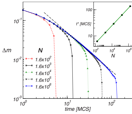
FIG. 3. Short time behavior of the order parameter \Delta m at h=h_{\text{sp}}^{(-)} for different system size N . The dashed (black) line corresponds to a power law fit to the N=1.6 \times 10^6 curve. Inset: t^* defined as the time for \Delta m to reach 10^{-3} vs N .
