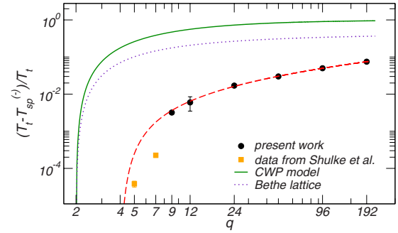
FIG. 12. (T_t - T_{\text{sp}}^{(-)}) / T_t vs q compared to mean-field predictions. Data for q = 5, 7 are from Ref. 15. The dashed (red) line is a fit to A \log^a(1+q-4) with A=0.0007 and a=2.81 .
