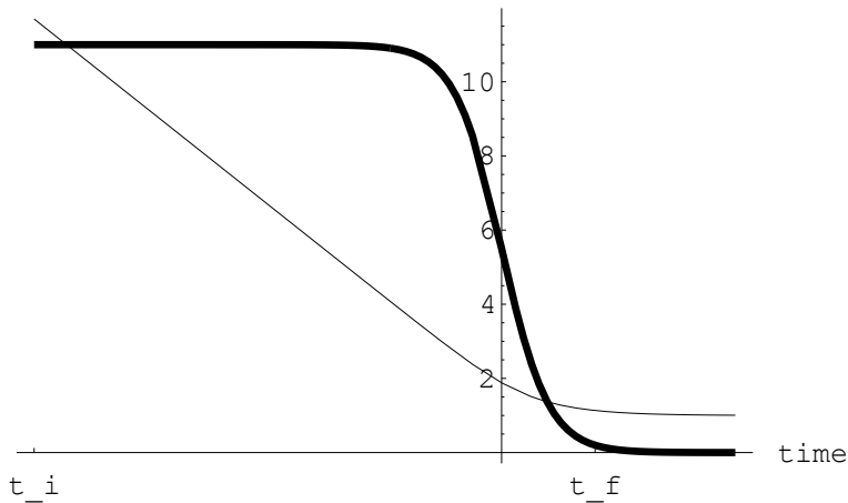
Figure 1: Temporal evolution of the condensate |\langle G^2 \rangle| (thick line) and the \epsilon -field (thin line), for the choice f(t) = -\beta^2 \tanh^2(\epsilon - 1) . The \langle G^2 \rangle scale has been adapted so that to visualize both graphs together.
