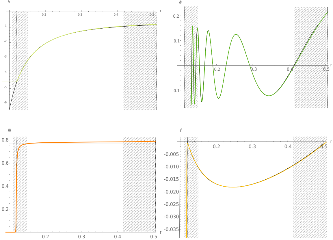
Figure 4. Full non linear numerical evolution (colour) and probe approximations (4.1) and (4.8)–(4.10) (black) of the profiles in the probe epoch. The dashed regions have been excluded from the fitting. That on the right of each plot interpolates to the polynomial approximation of the previous subsection, while the one on the left connects to the collapse of the Einstein-Rosen bridge described below. The dashed line at large r corresponds to the black hole horizon, while that at small r signals the position of the would-be Cauchy horizon. The values of the parameters correspond to the black hole shown in figure 1 (left).
