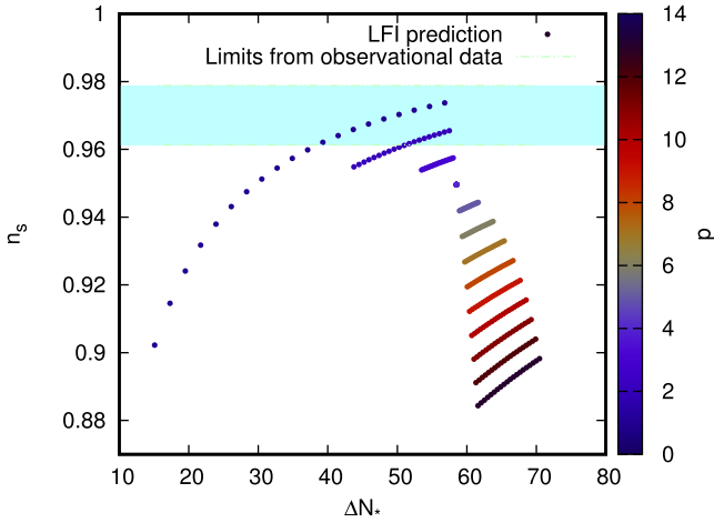
Fig. 4. The predicted spectral index n_s as a function of \Delta N_* with varying parameter p for the LFI potential in the standard framework. The shadowed region corresponds to the estimated n_s at 2\sigma CL using Planck 2015 + BAO data set.
