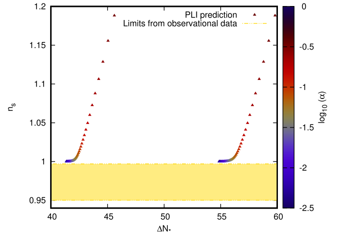
Fig. 11. The predicted spectral index n_s as a function of \Delta N_* with varying parameter \alpha for the PLI potential in Wigner's scheme. The shadowed region corresponds to the estimated n_s at 2\sigma CL using Planck 2015 + BAO data set.
