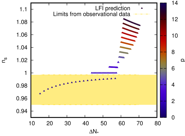
Fig. 3. The predicted spectral index n_s as a function of \Delta N_* with varying parameter p for the LFI potential in Wigner's scheme. The shadowed region corresponds to the estimated n_s at 2\sigma CL using Planck 2015 + BAO data set.
