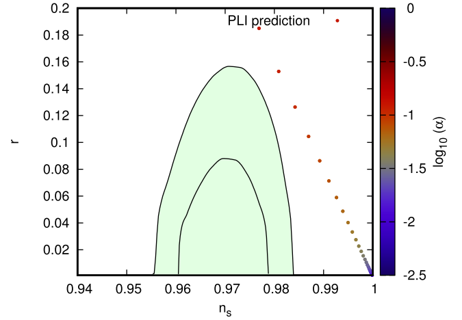
Fig. 10. The predicted n_s and r as a function of \Delta N_* with varying parameter \alpha for the PLI potential in the standard framework. The shadowed region corresponds to the marginalized 68% and 95% CL regions for n_s and r from Planck 2015 + BAO data set.
