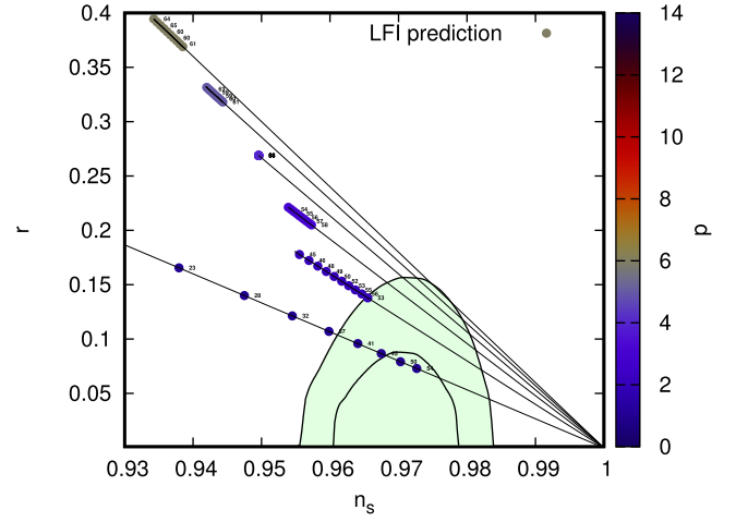
Fig. 5. The predicted n_s and r as a function of \Delta N_* with varying parameter p for the LFI potential in the standard framework. The shadowed region corresponds to the marginalized 68% and 95% CL regions for n_s and r from Planck 2015 + BAO data set.
