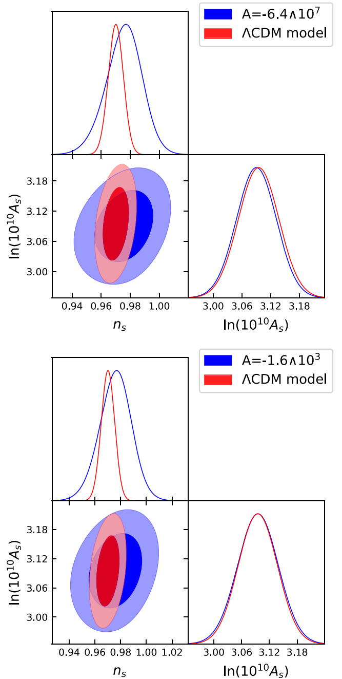
Fig. 2. 68% and 95% two dimensional confidence regions and posterior probability density of n_s and A_s for two values of A using Planck 2015 + BAO data set. We also show the same confidence regions of the \Lambda CDM model (red) in the two plots. Other values of A exhibit the same behavior. (For interpretation of the references to color in this figure legend, the reader is referred to the web version of this article.)
