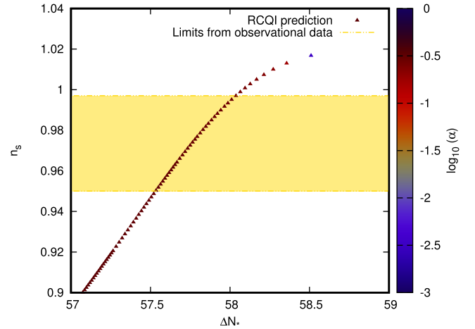
Fig. 6. The predicted spectral index n_s as a function of \Delta N_* with varying parameter \alpha for the RCQI potential with \omega_{reh} = -\frac{1}{3} in Wigner's scheme. The shadowed region corresponds to the estimated n_s at 2\sigma CL using Planck 2015 + BAO data set.
