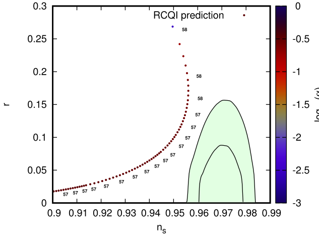
Fig. 8. The predicted n_s and r as a function of \Delta N_* with varying parameter \alpha for the RCQI potential with \omega_{reh} = -\frac{1}{3} in the standard framework. The shadowed region corresponds to the marginalized 68% and 95% CL regions for n_s and r from Planck 2015 + BAO data set.
