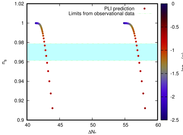
Fig. 9. The predicted spectral index n_s as a function of \Delta N_* with varying parameter \alpha for the PLI potential in the standard framework. The shadowed region corresponds to the estimated n_s at 2\sigma CL using Planck 2015 + BAO data set.
