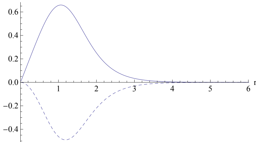
Figure 1: The electric (solid line) and magnetic (dashed line) fields in the region \alpha > 0, \beta < \beta_{crit} , with \alpha = 1, \beta_{crit} = 0.0625 and \beta = 0.04 . As in the relativistic Chern-Simons-Higgs model, the magnetic and electric fields form a ring surrounding the vortex core.
