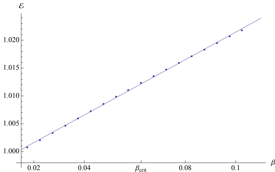
Figure 4: The energy as a function of \beta for \alpha = 1, \beta_{\text{crit}} = 0.0625
