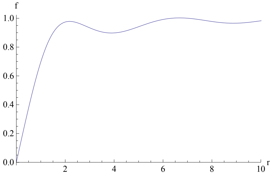
Figure 6: The Higgs field profile in the region \alpha < 0 , \beta > \beta_{crit} , with \alpha = -0.2 , \beta_{crit} = 0.0025 and \beta = 0.25 .
