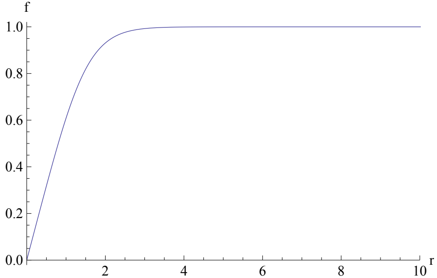
Figure 2: The Higgs field profile in the region corresponding to \alpha > 0 , \beta < \beta_{\text{crit}} . ( \alpha = 1 , \beta_{\text{crit}} = 0.0625 and \beta = 0.04 )
