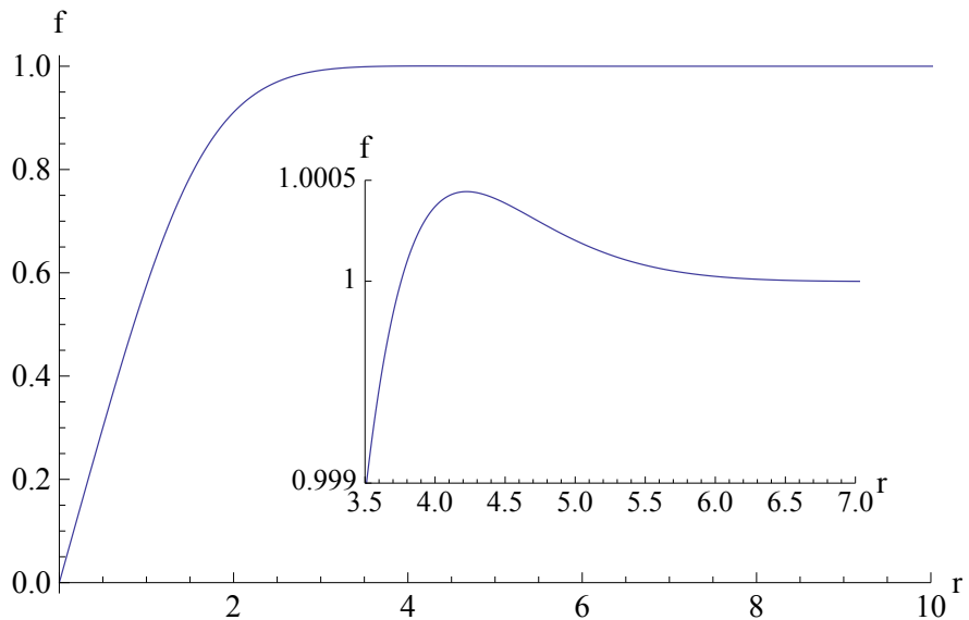
Figure 3: The Higgs field profile in the region \alpha > 0 , \beta > \beta_{\text{crit}} . We have chosen \alpha = 1 , \beta_{\text{crit}} = 0.0625 and \beta = 0.2 . The inset shows a zoom of the region where f overshoots its vev and comes back to it, as is characteristic of an underdamped behavior.
