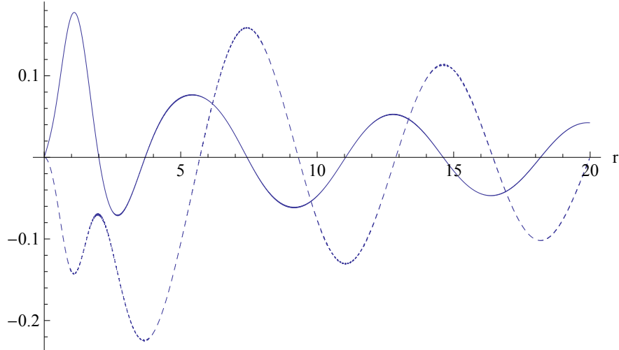
Figure 5: The electric (solid line) and magnetic (dashed line) fields in the region \alpha < 0 , \beta > \beta_{crit} , with \alpha = -0.2 , \beta_{crit} = 0.0025 and \beta = 0.25 .
